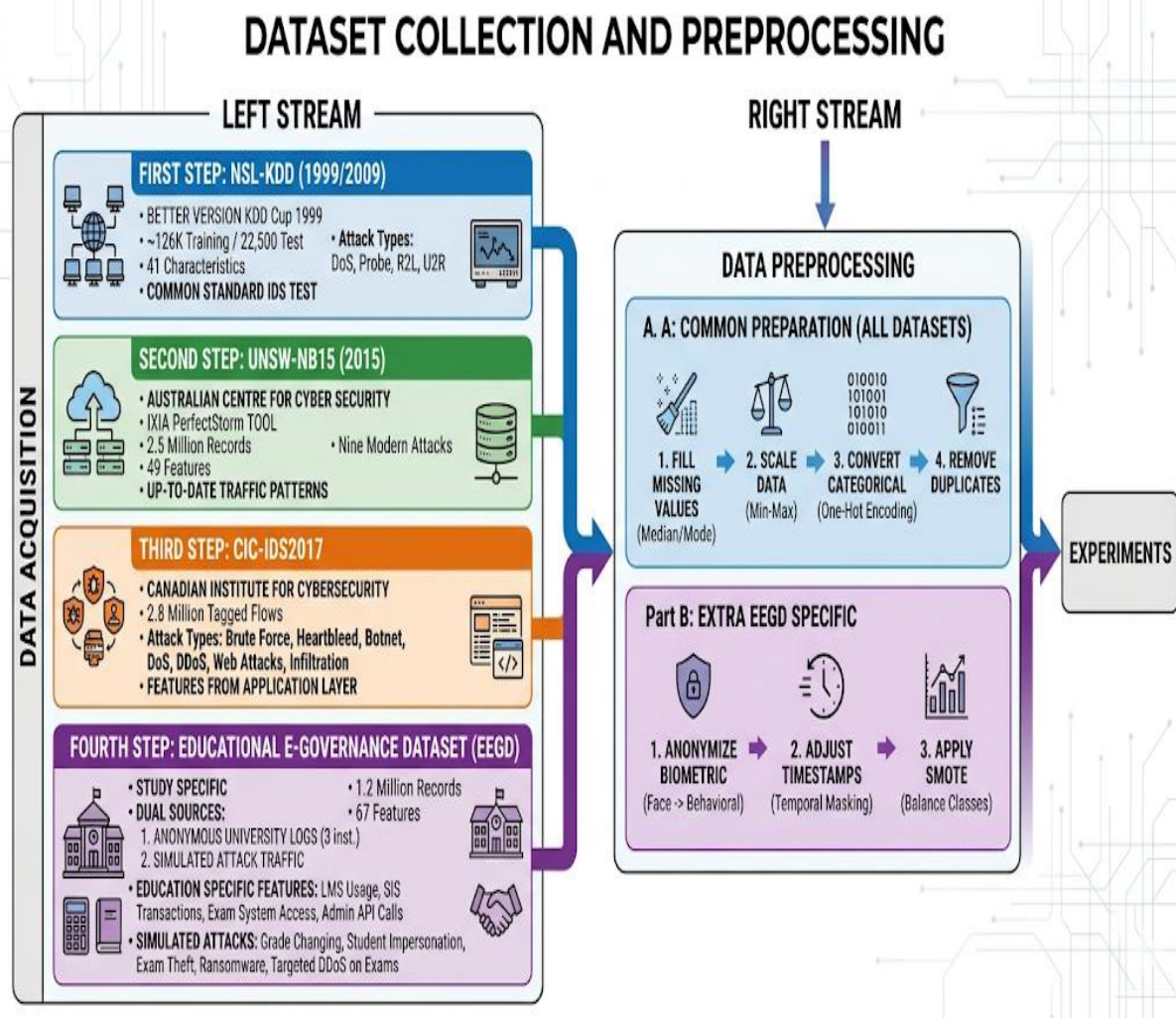
Figure 1: BASE_ECG Dataset collection and Processing's
