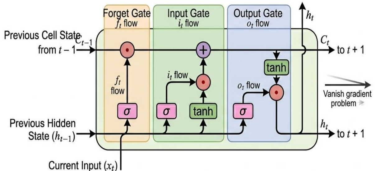
Figure 1: LSTM Cell Computation Graph and Gated Architecture
