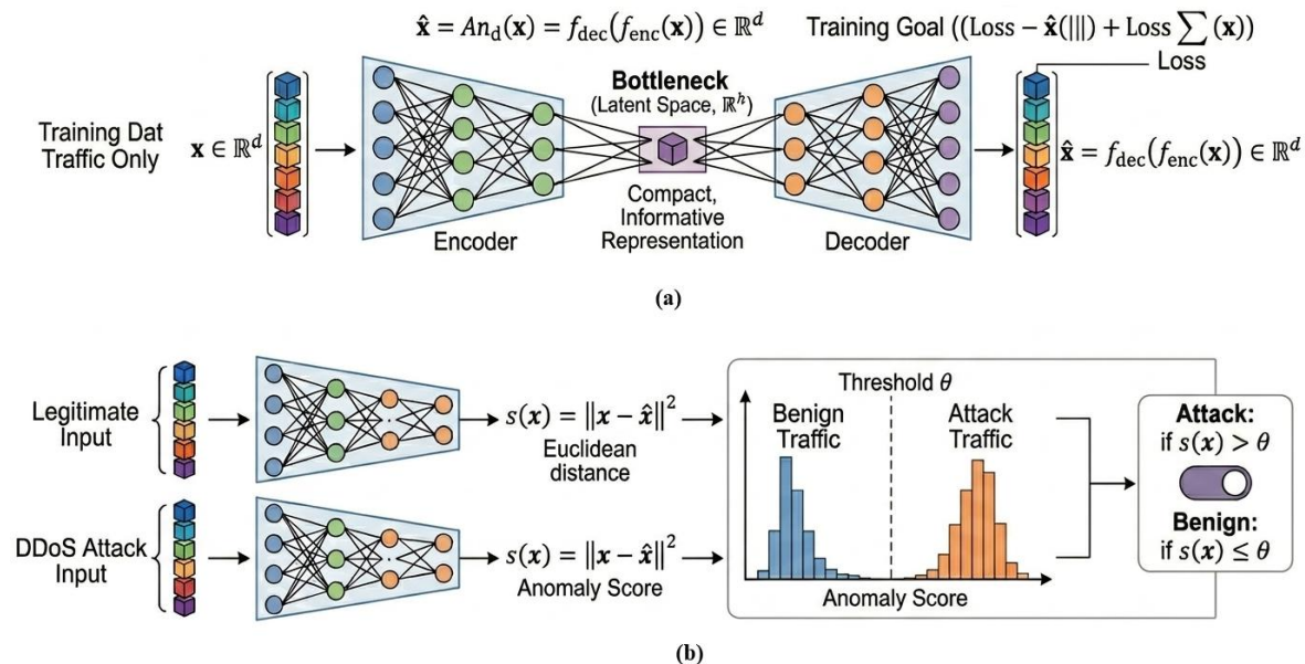
Figure 2: Autoencoder Anomaly Scoring for DDoS Detection: (a) Architecture and the Bottleneck Effect (b) DDoS Anomaly Scoring and Decision Logic
